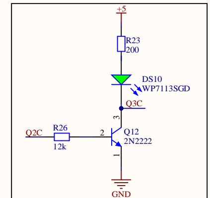
Stage 5: LED Driver
