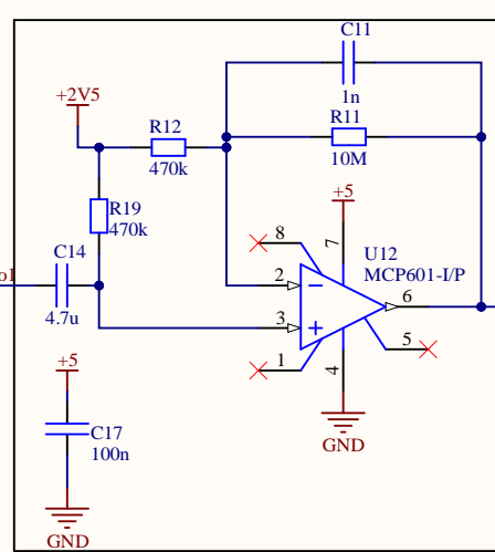
Stage 2: High pass filter and gain
