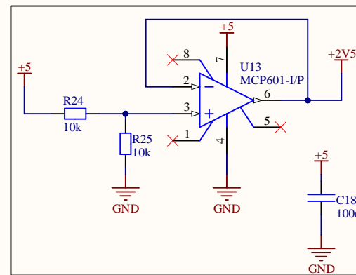
Unity Gain Amplifier - Voltage Reference for 2.5V
