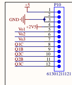
Debug Connector
