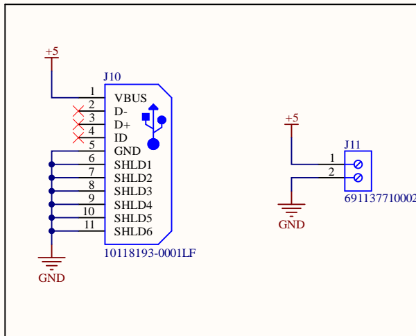
Power: USB and Terminal Block
