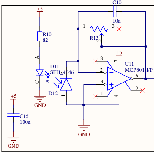
Stage 1: Transresistance Amplifier (w/ LP response)
