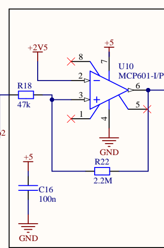
Stage 3: Comparator
